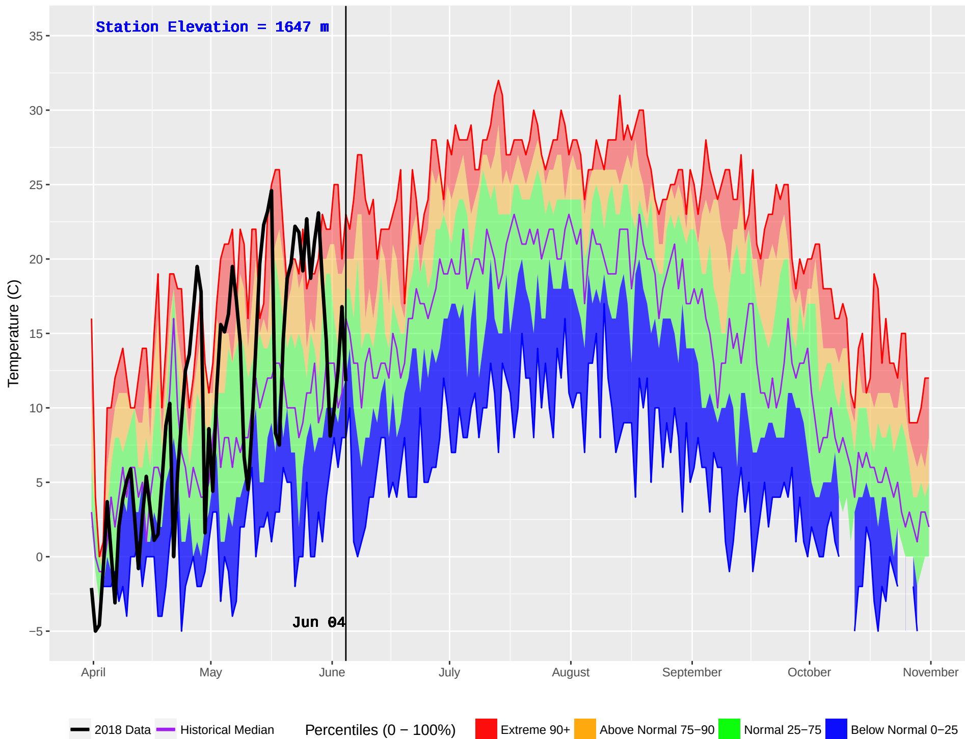
ROUND PRAIRIE (788) : Historical (2001–2016) and Current (2018) Noon Temperature
