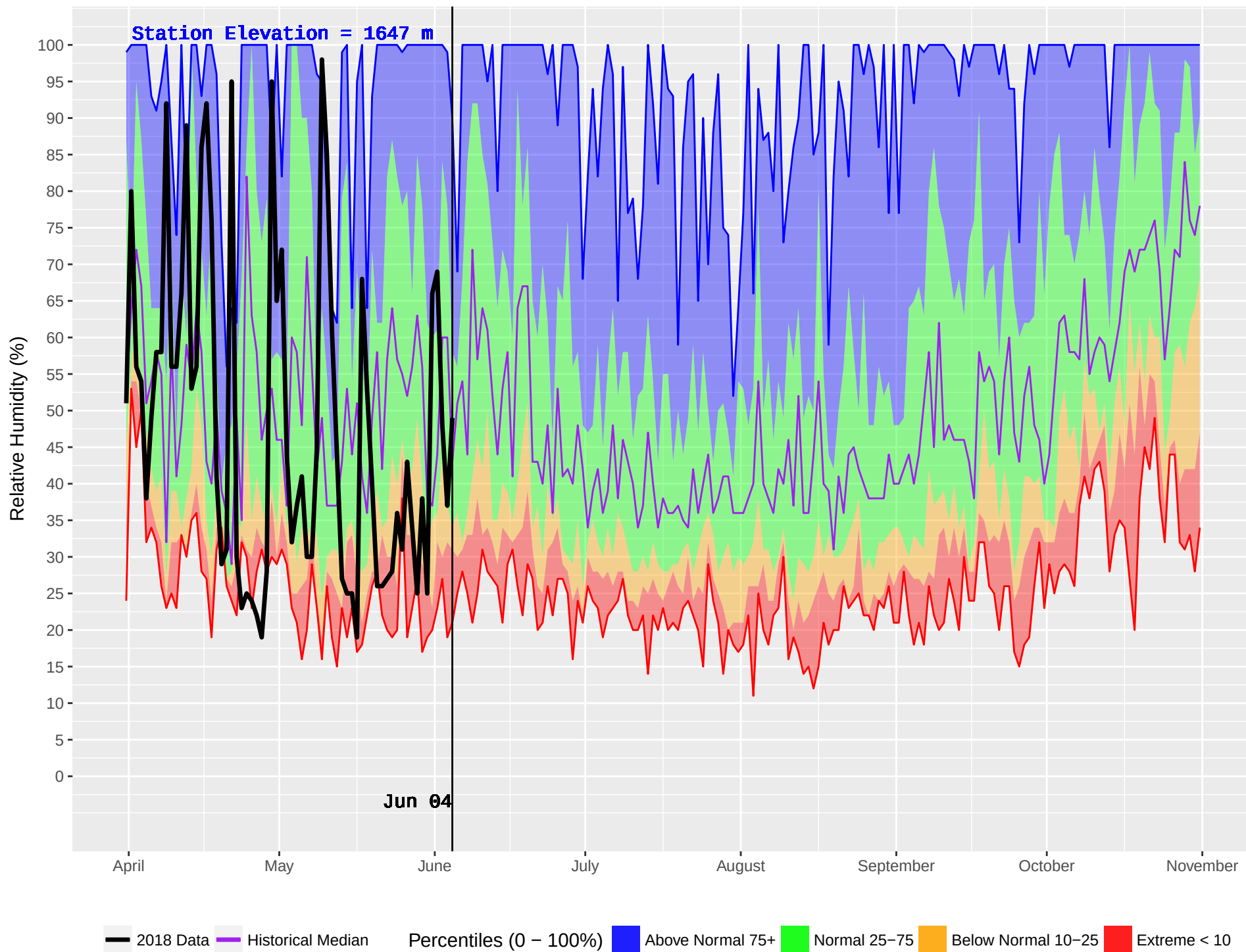
ROUND PRAIRIE (788) : Historical (2001–2016) and Current (2018) Noon Relative Humidity
