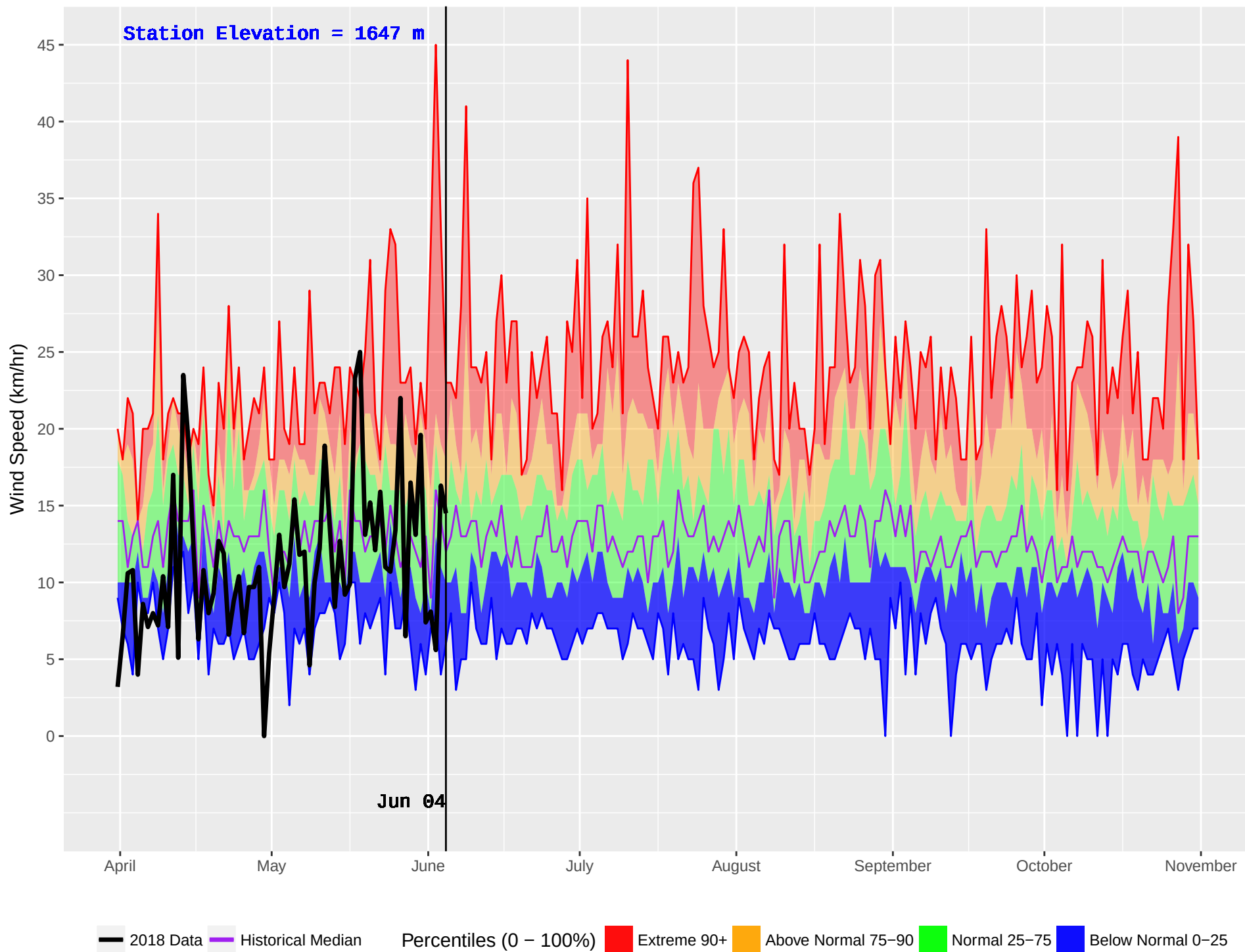
ROUND PRAIRIE (788) : Historical (2001–2016) and Current (2018) Noon Wind Speed
