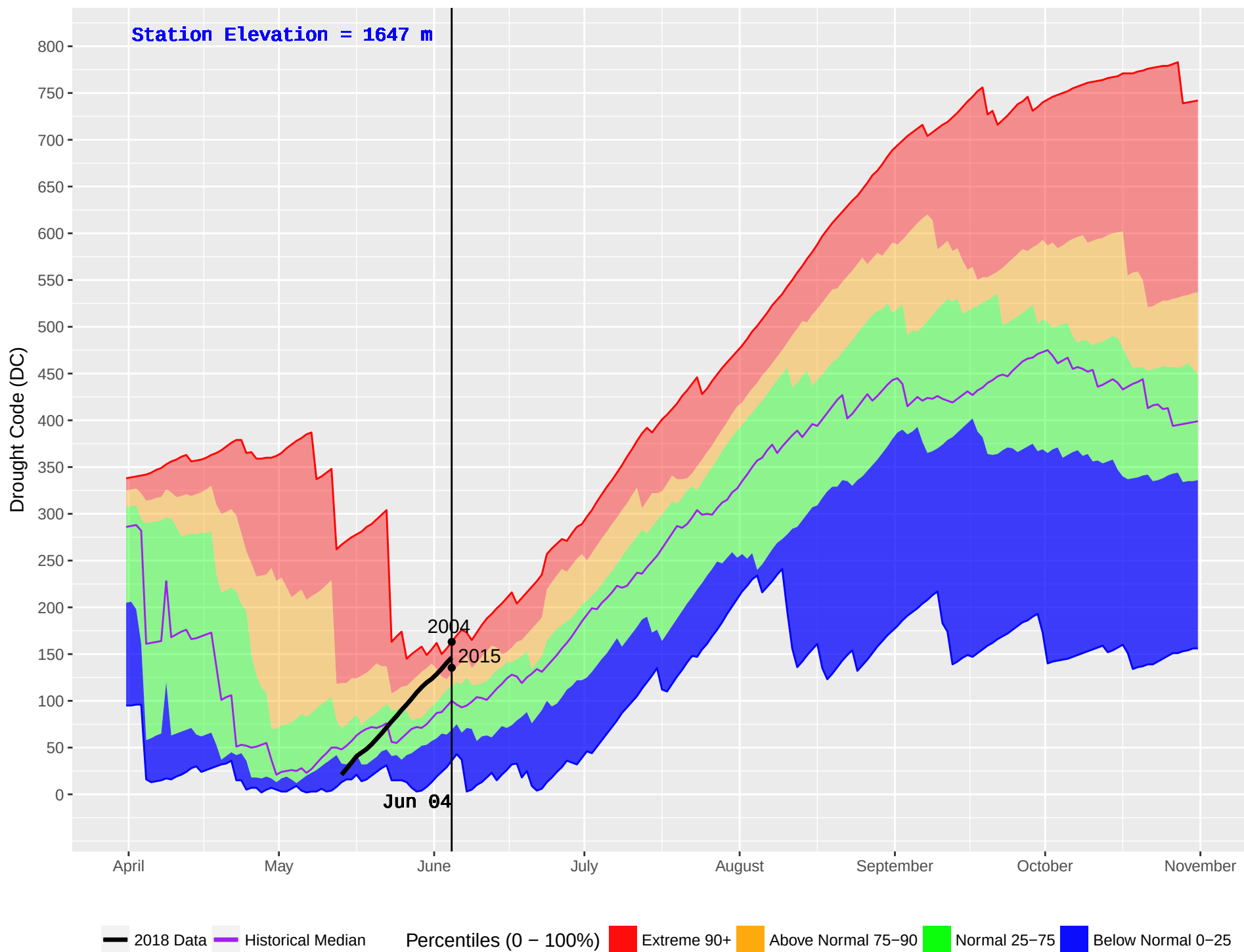
ROUND PRAIRIE (788) : Historical (2001–2016) and Current (2018) Noon Drought Code (DC)
