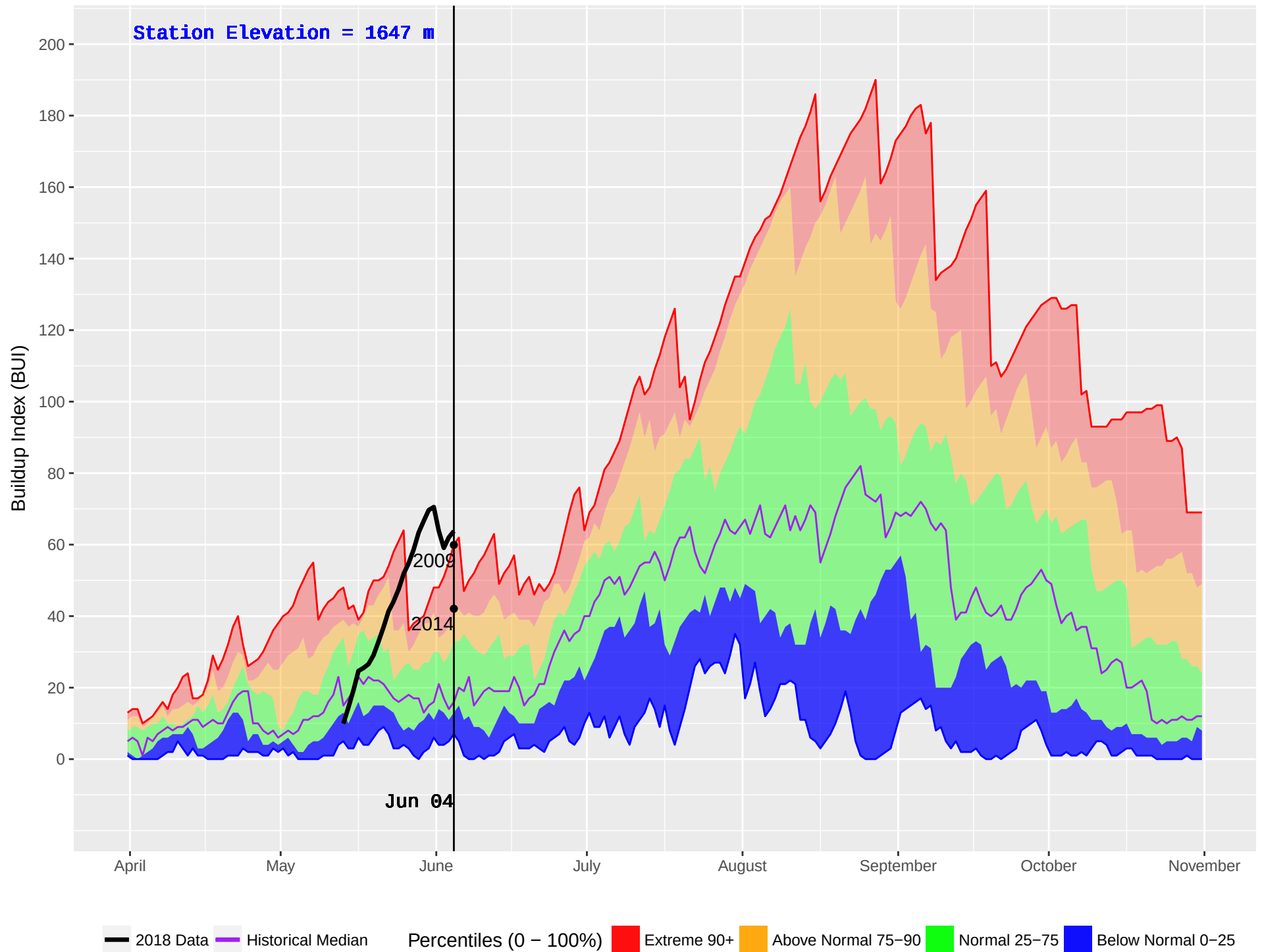
ROUND PRAIRIE (788) : Historical (2001–2016) and Current (2018) Noon Buildup Index (BUI)
