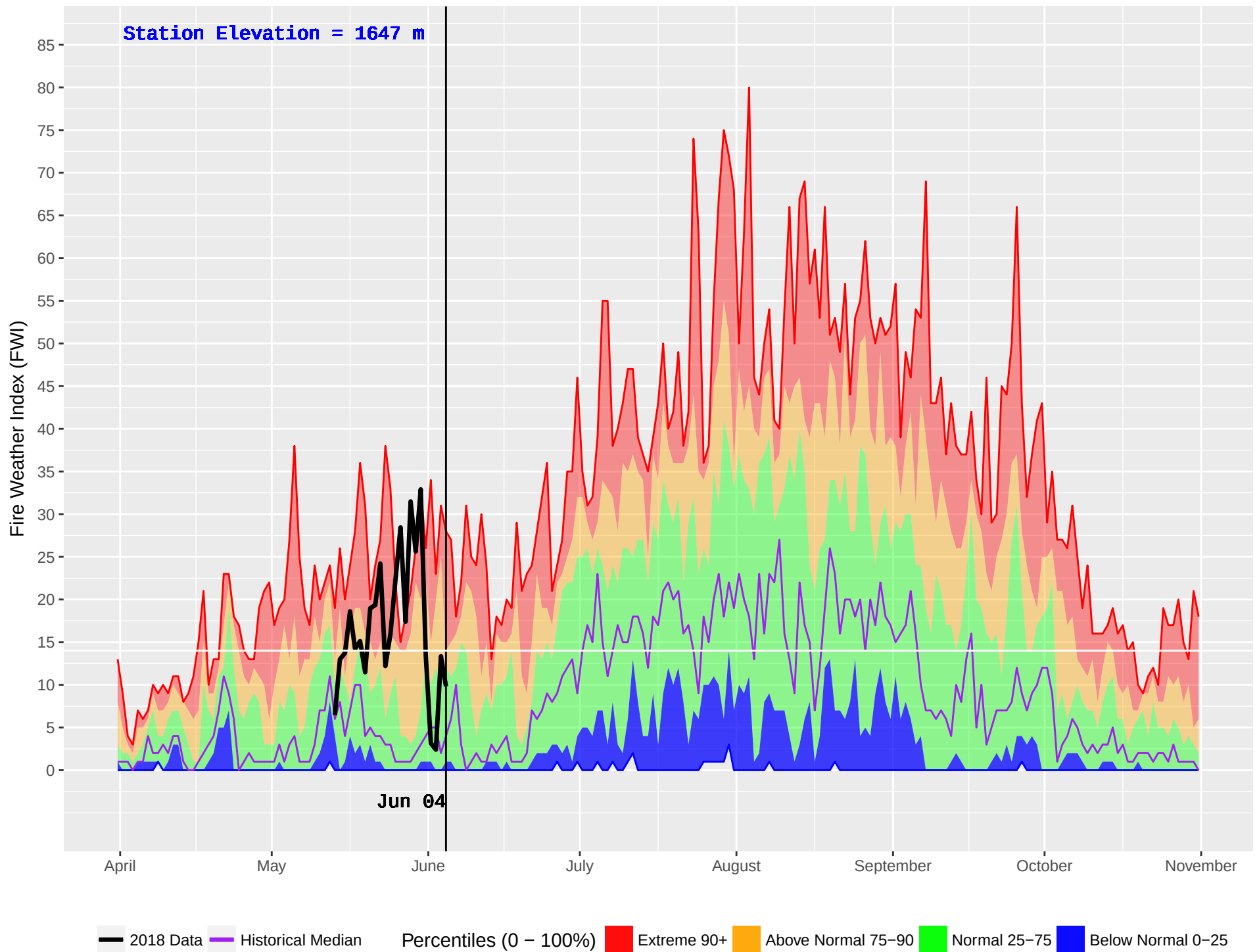
ROUND PRAIRIE (788) : Historical (2001–2016) and Current (2018) Noon Fire Weather Index (FWI)
