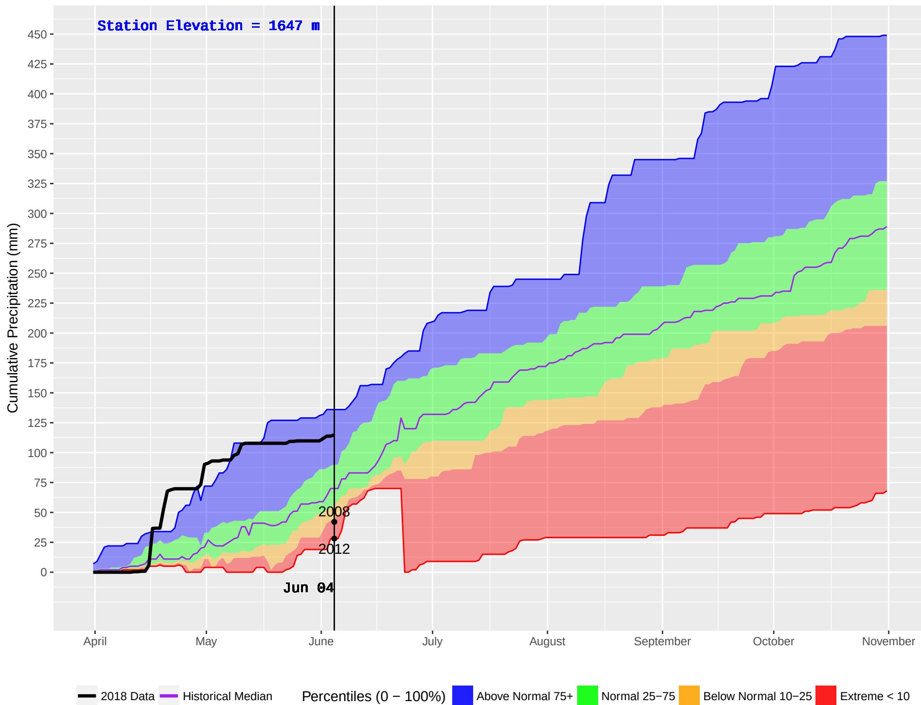
ROUND PRAIRIE (788) : Historical (2001–2016) and Current (2018) Noon Cumulative Precipitation
